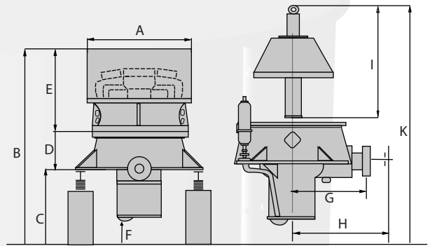
VH-Type
